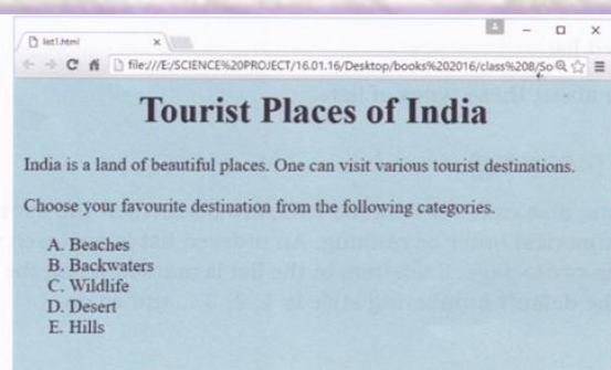
Output Window (<OL> tag and its type attribute)
